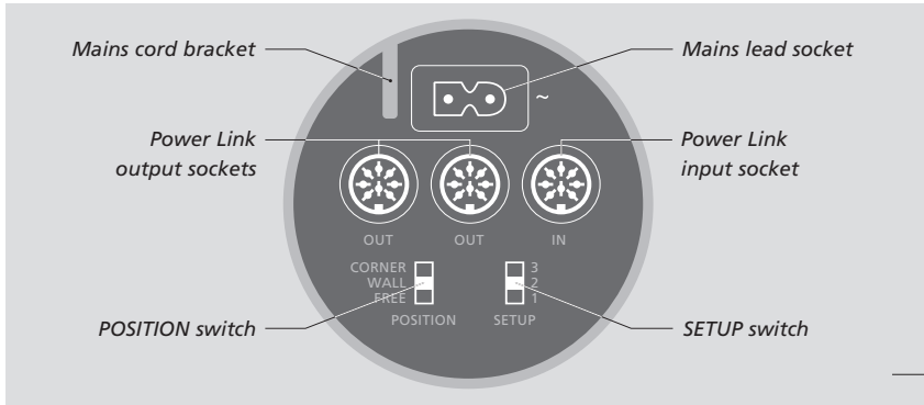
Rear view of BeoLab 2 showing the location of the socket and switch panel.
