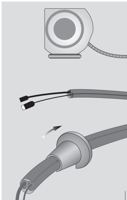
Cable cover: Use the enclosed tool to seal the cable cover when you have placed both the mains cord and the Power Link cable inside it.
